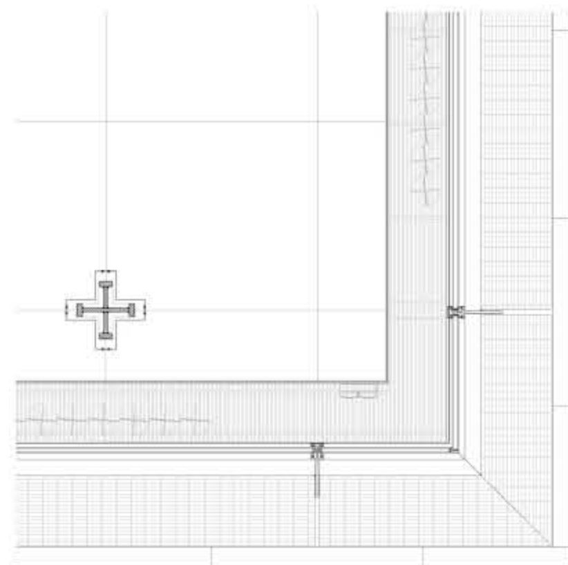
Horizontal Section
